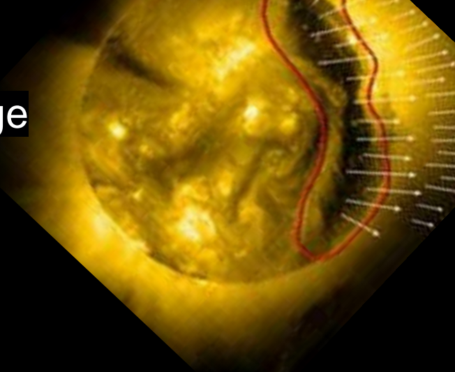
Open magnetic field lines flow from coronal holes
